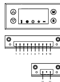
Figure 3 - Wiring interface with customer circuit
