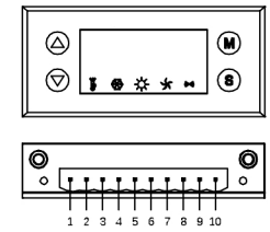
Figure 3 - Wiring interface with customer circuit
