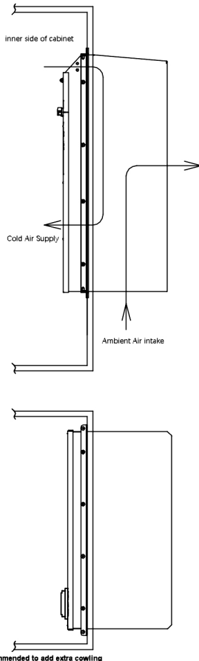
Figure 1 - Installation tips if extra cowling needed by customer
