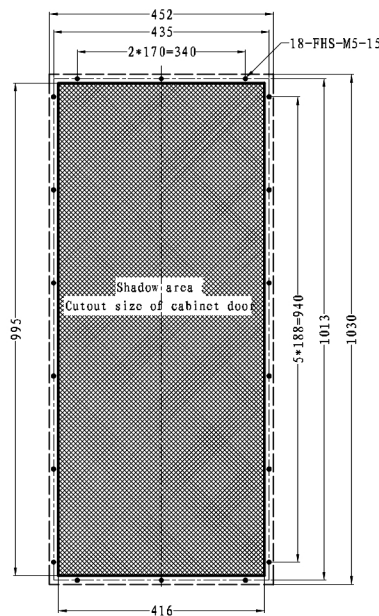
Blue dashed rectangle: Air conditioner projected dimension on door (1030x452mm)
