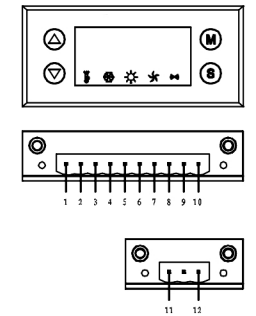
Figure 3 - Wiring interface with customer circuit
