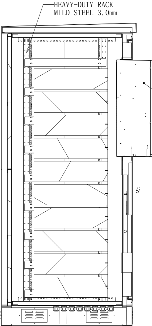
SECTION B-B
