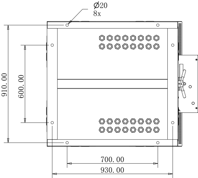
ANCHORING LAYOUT
